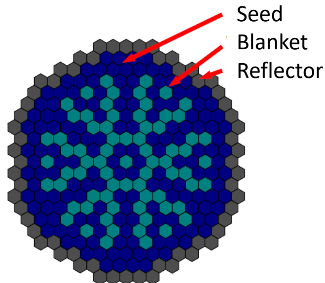
Super FR core configuration
