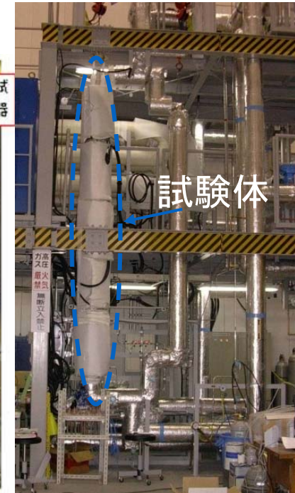
Turbulent mixing cross-flow test (Kyushu U.)
